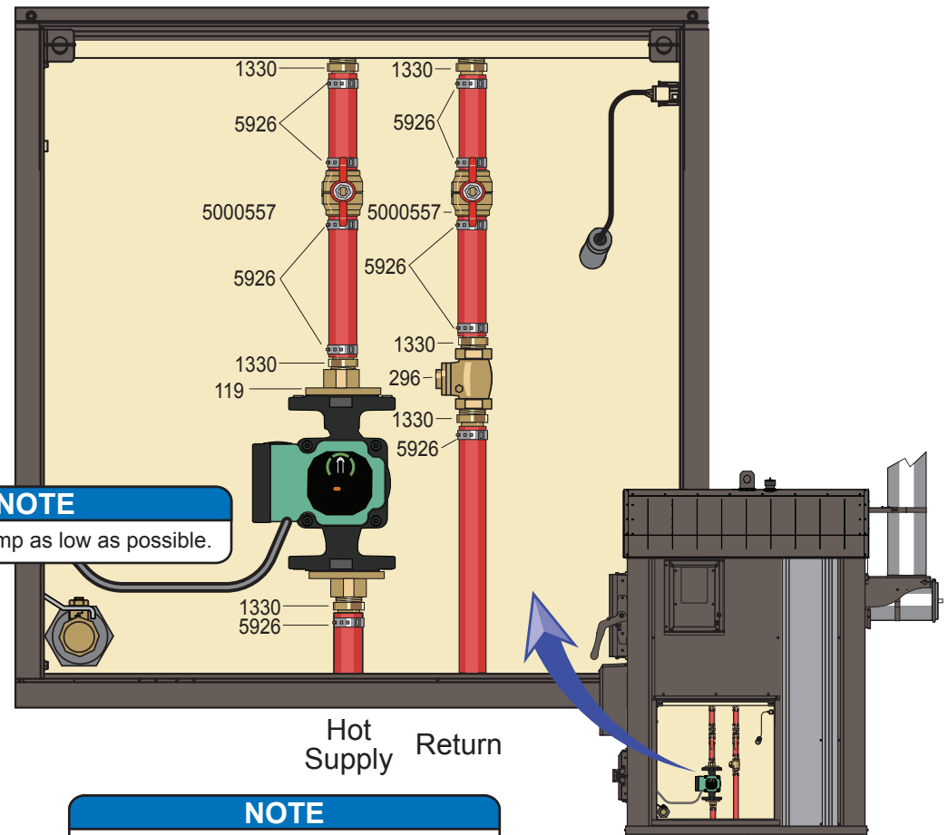
3xx/5xx Pump Panel
